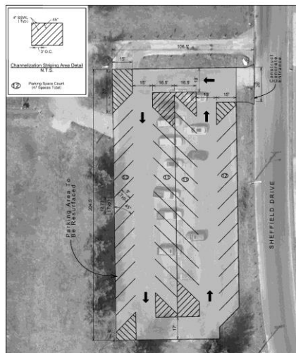
2018 Citywide Facilities Paving - Site 4 WEST HILLS PARK 7624 SHEFFIELD DRIVE City of Knoxville Dept. of Engineering Scale: 1" = 30'
