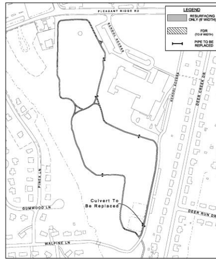
2018 Citywide Facilities Paving - Site 1 Northwest Middle School Greenway City of Knoxville Dept. of Engineering Scale: N.T.S.
