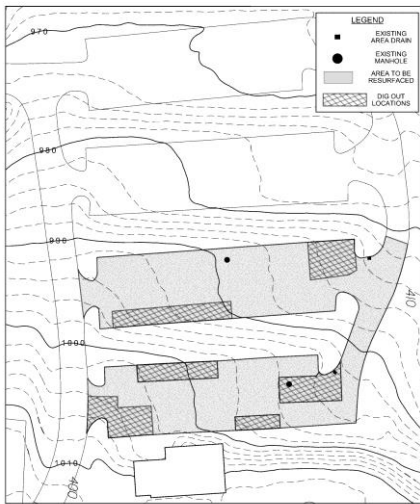
2018 Citywide Facilities Paving - Site 3 WEST HILLS PARK 400 NORTH WINSTON ROAD Scale: 1" = 50'
