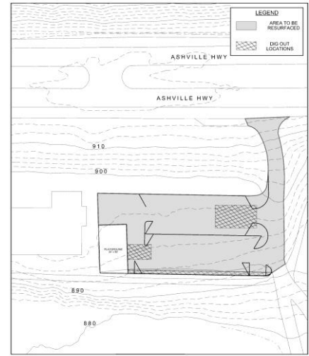
2018 Citywide Facilities Paving - Site 2 MILTON ROBERTS RECREATION CENTER City of Knoxville Dept. of Engineering Scale: 1" = 50'
