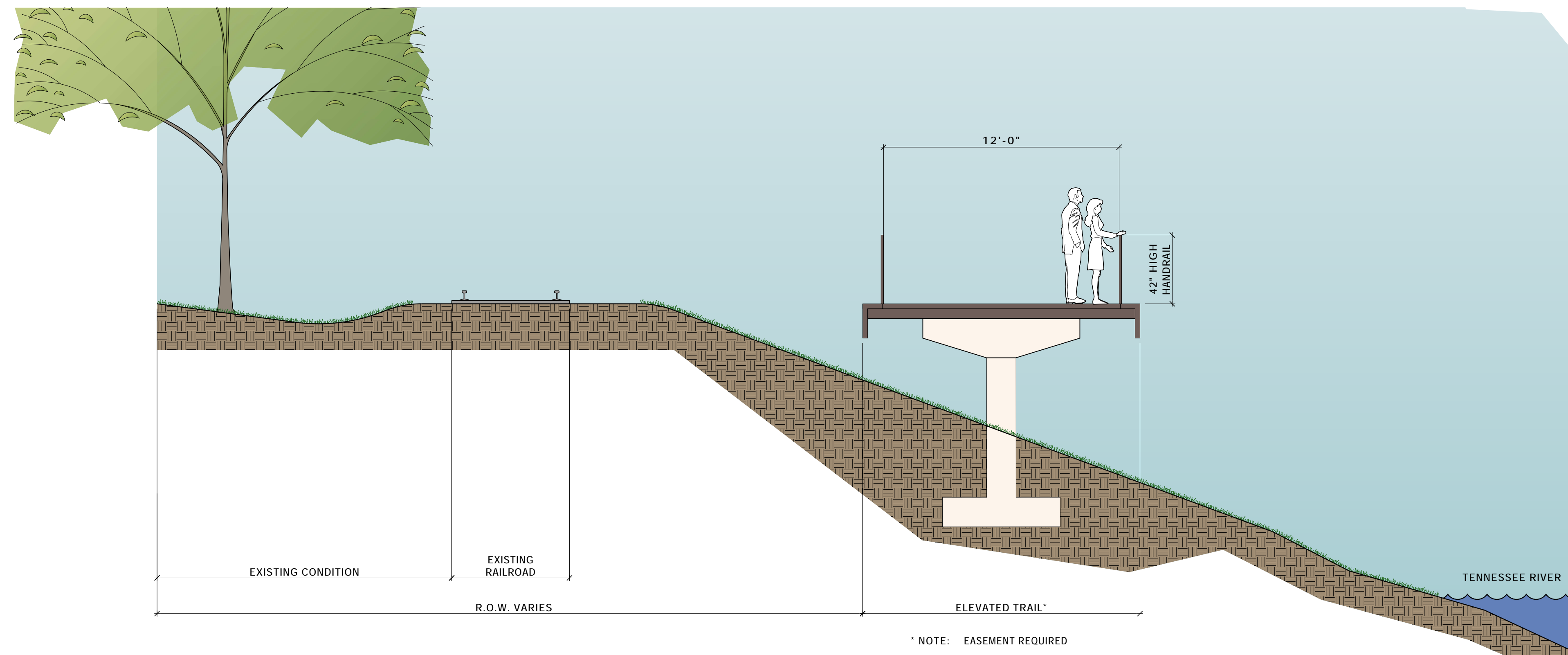
6 TYPICAL TRAIL ON STRUCTURE SECTION (2 SEGMENTS, TOTAL 0.67 MI.) SCALE: 1/4"=1'-0"
