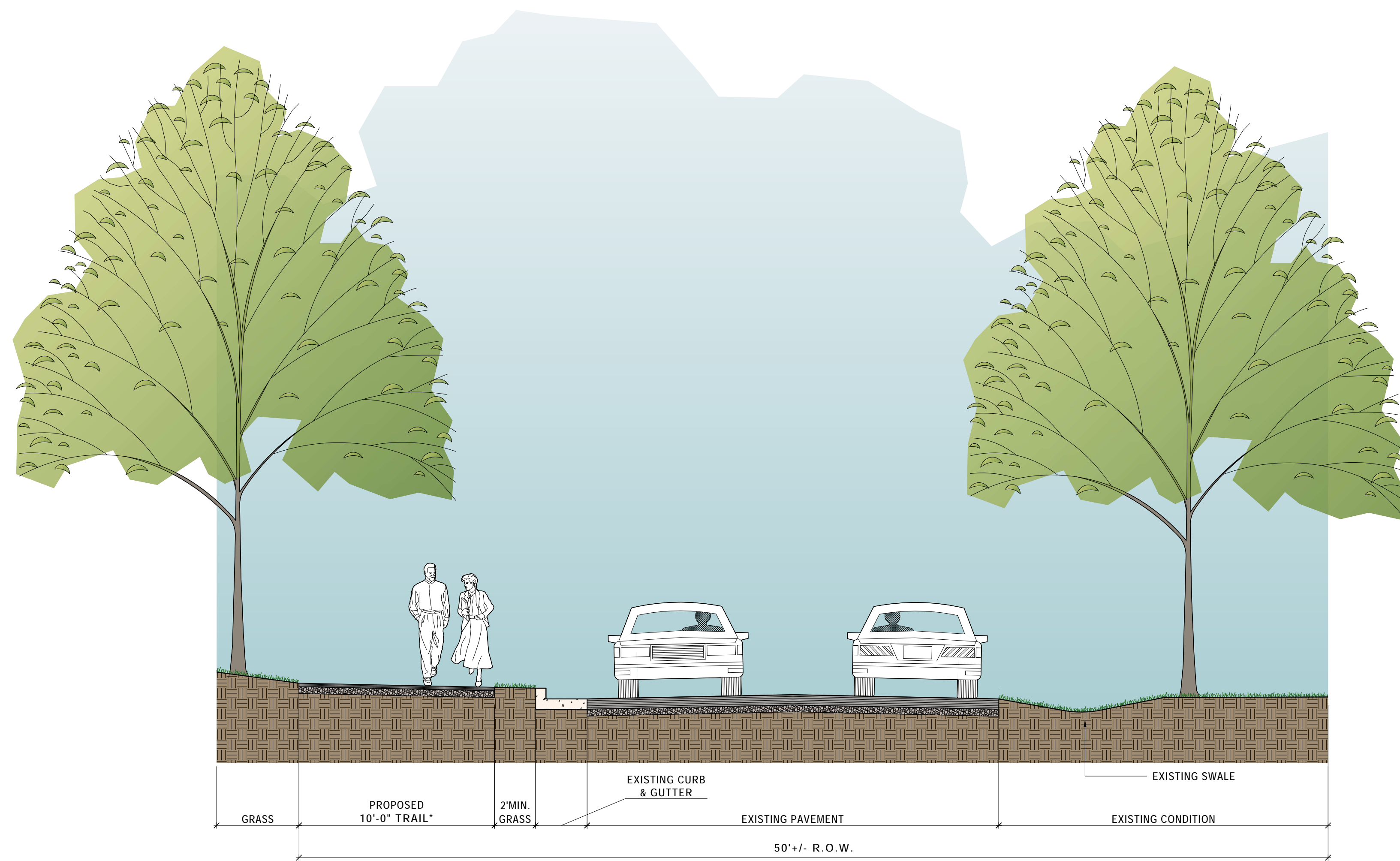
19 LYONS VIEW TYPICAL TRAIL SECTION SCALE: 1/4"=1'-0" * EXISTING SIDEWALK REMOVAL REQUIRED
