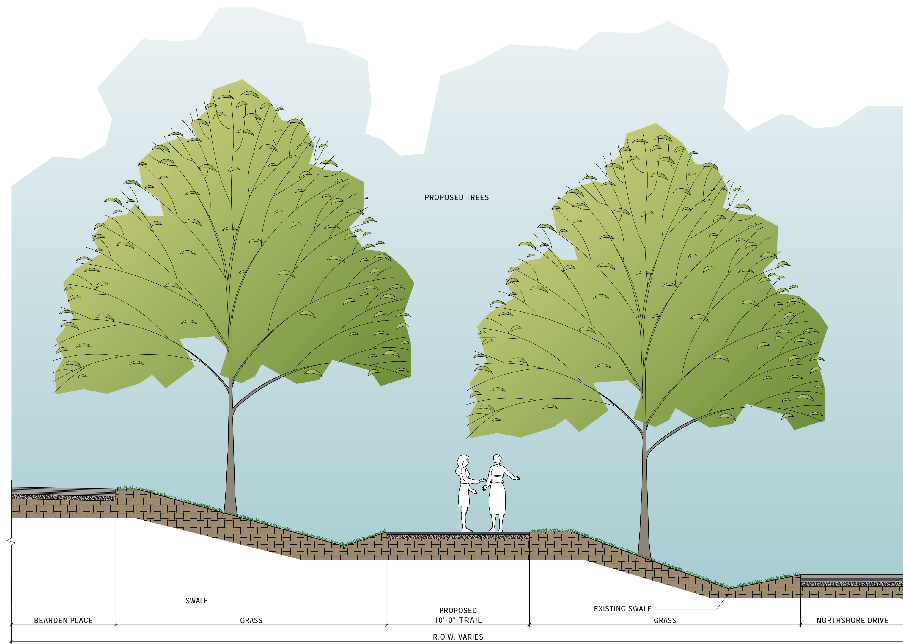
4 TRAIL ALONG NORTHSHORE DRIVE SCALE: 1/4"=1'-0"
