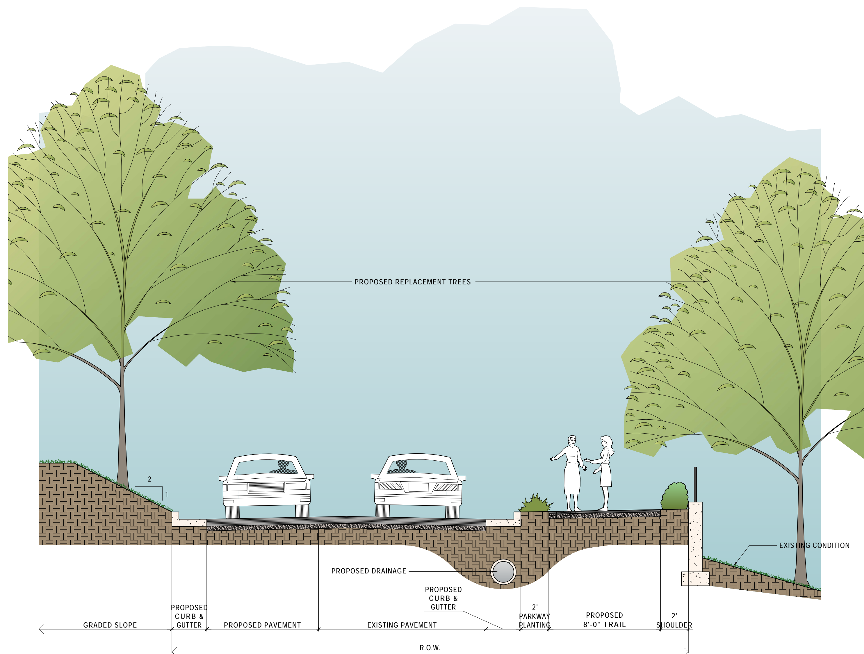
6 NEIGHBORHOOD CONNECTOR TYPE 2 @ TOOLE DRIVE SCALE: 1/4"=1'-0"
