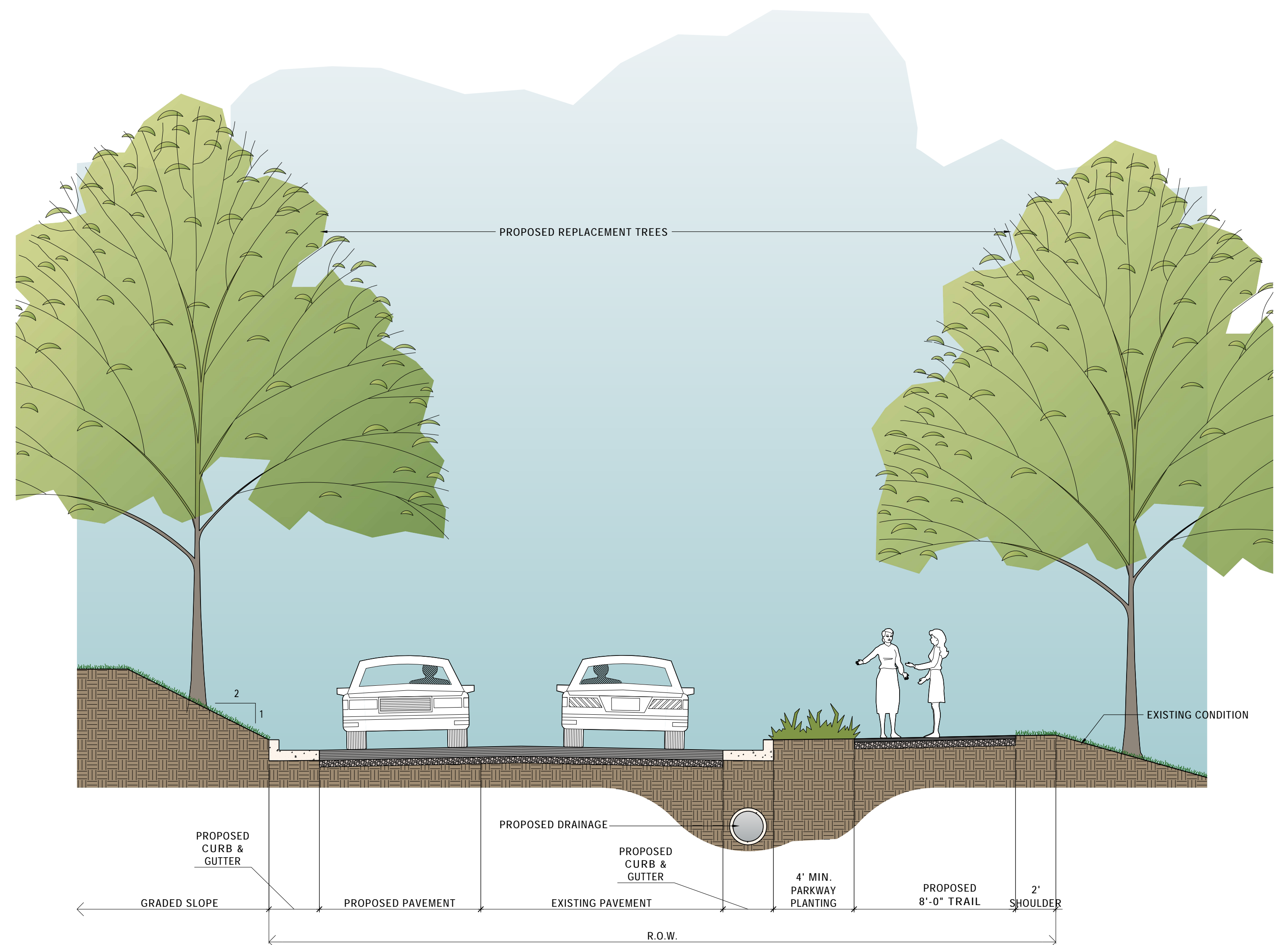
5 NEIGHBORHOOD CONNECTOR TYPE 1 @ TOOLE DRIVE SCALE: 1/4"=1'-0"
