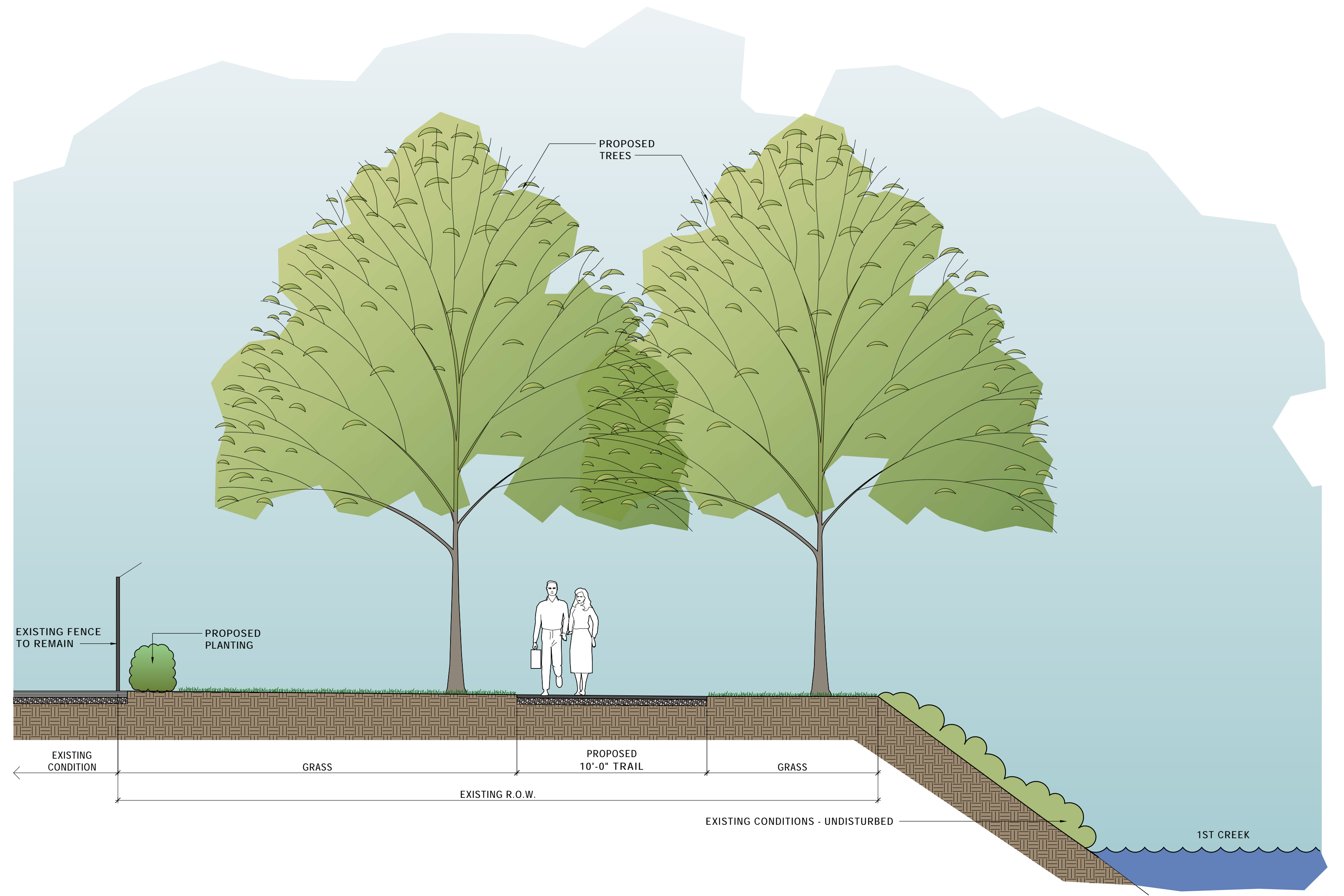
3 TRAIL ALONG FIRST CREEK @ KAT SCALE: 1/4"=1'-0"
