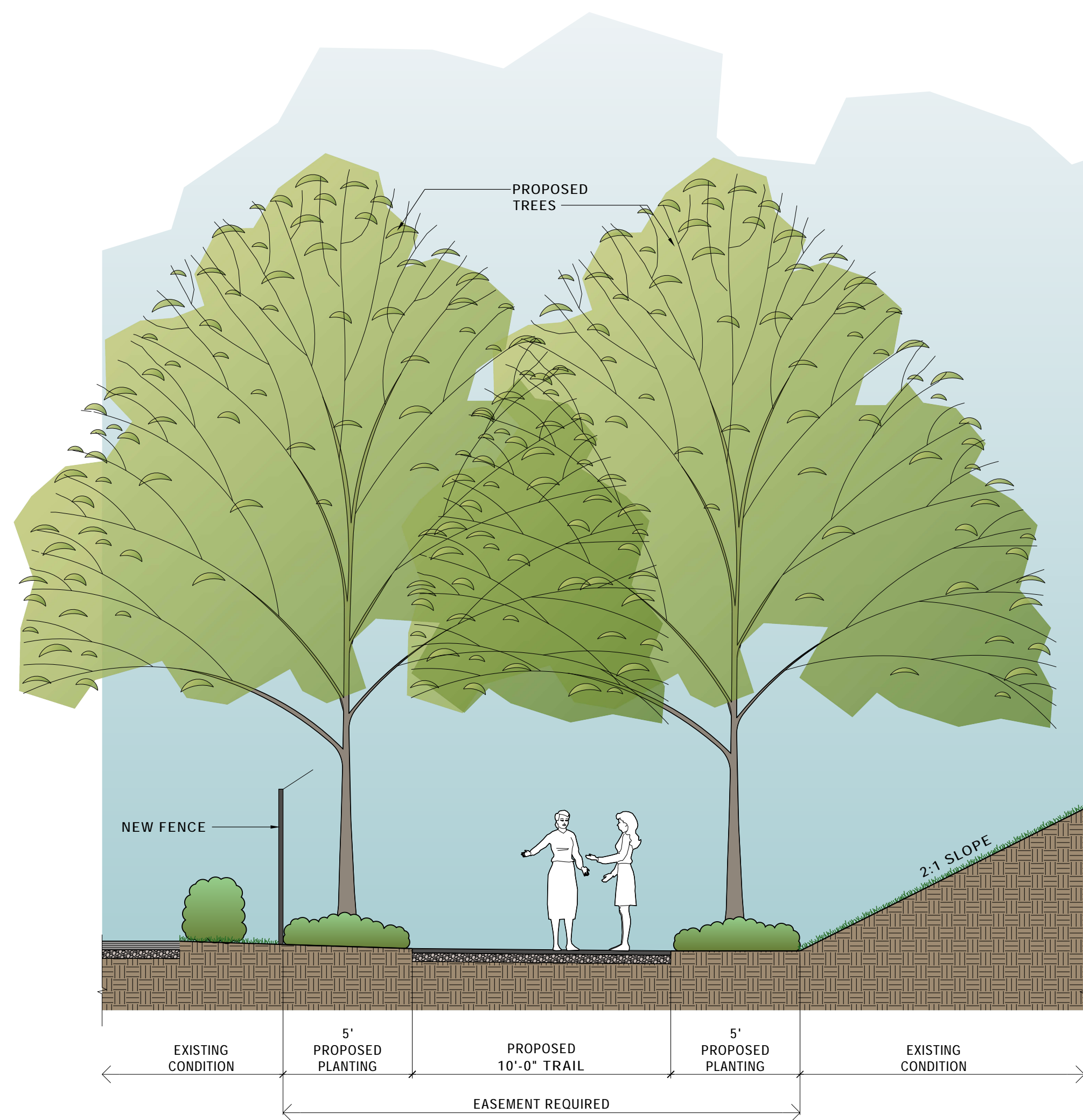
4 TRAIL ON GRADE SCALE: 1/4"=1'-0"
