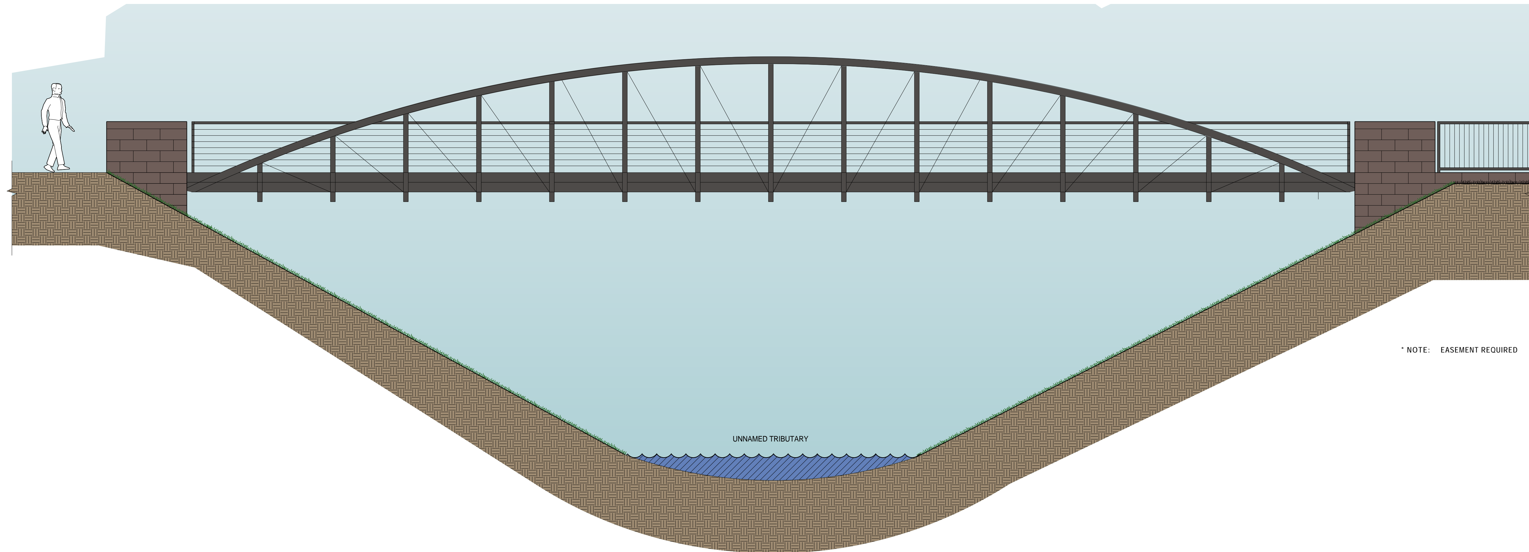
9 BRIDGE AT UNNAMED TRIBUTARY (60 FT.) SCALE: 1/4" = 1'-0"
