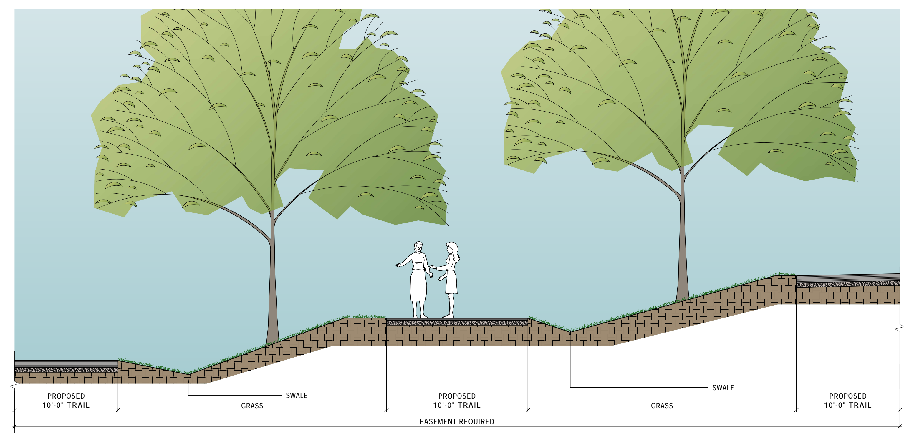
10 TYPICAL TRAIL ON SLOPE SCALE: 1/4" = 1'-0"
