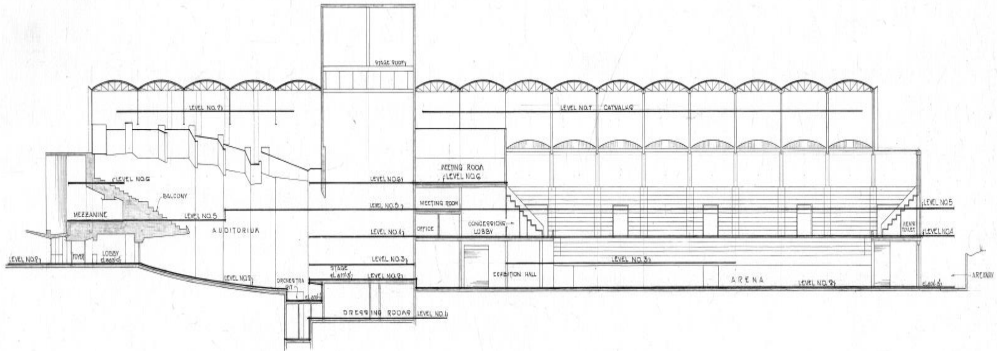
SCHEMATIC CROSS-SECTION
