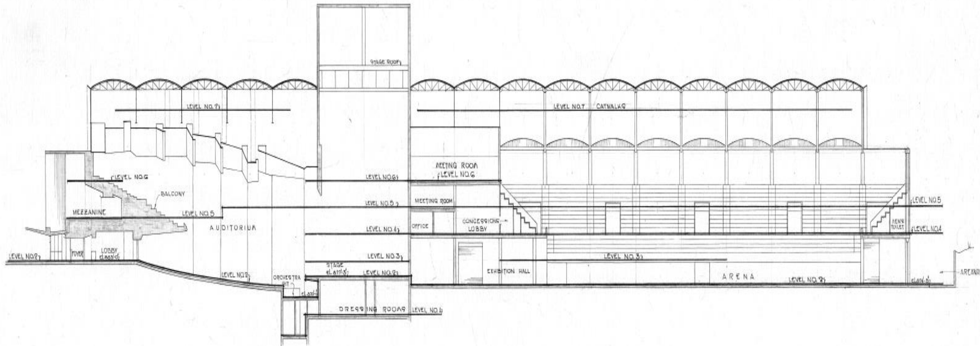
SCHEMATIC CROSS-SECTION
