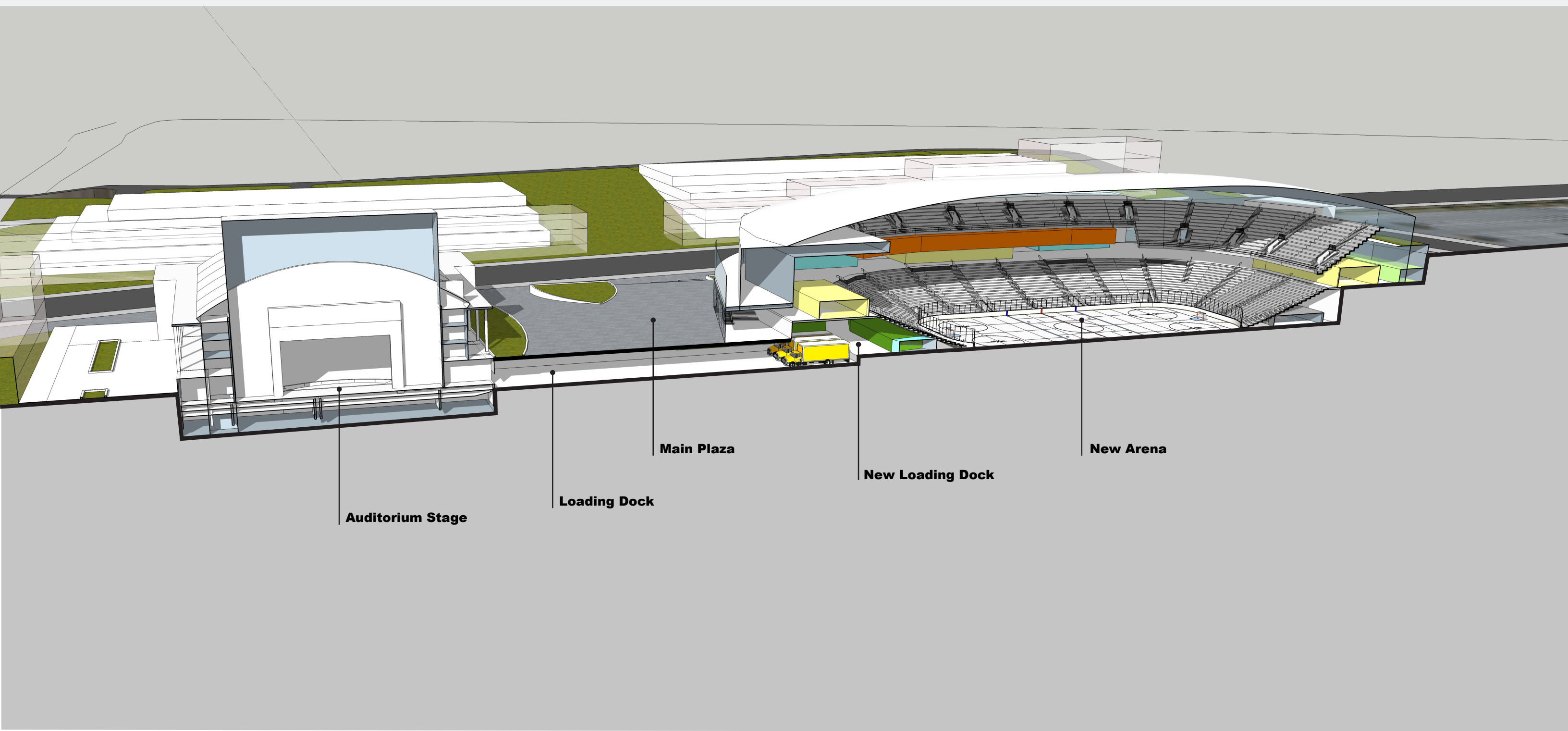
OPTION 1-EAST-WEST SECTION
