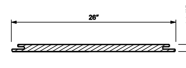
CROSS SECTION
