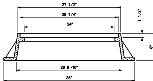
CROSS SECTION
