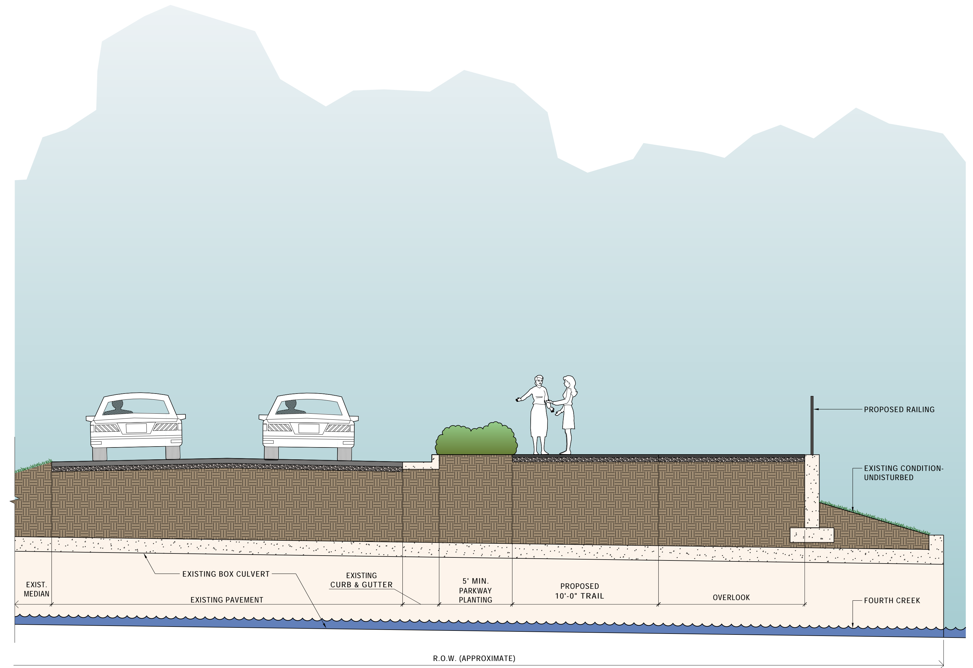
7 SIDE PATH WITH PARKWAY ALONG MIDDLEBROOK PIKE @ 4TH CREEK OVERLOOK SCALE: 1/4"=1'-0"
