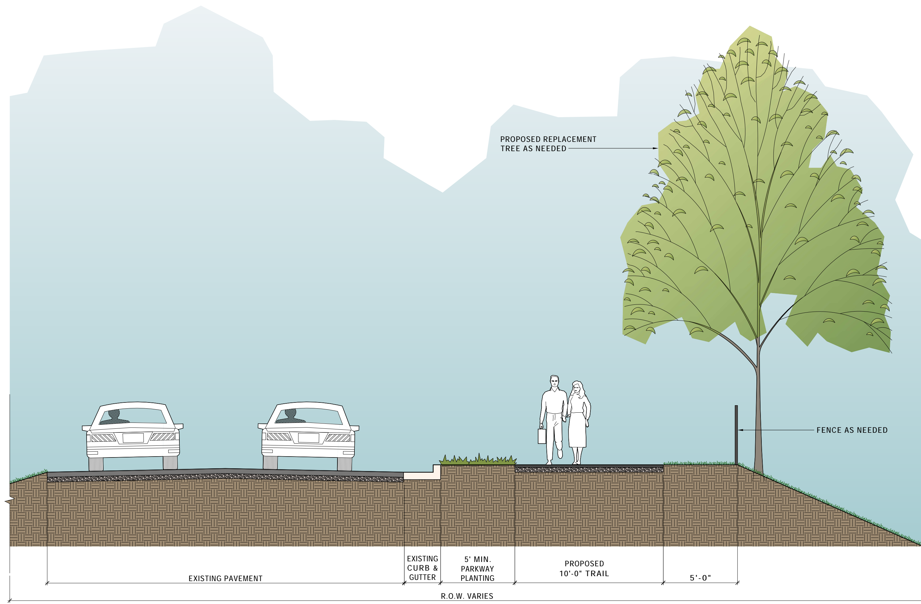
8 SIDE PATH WITH PARKWAY SECTION ALONG MIDDLEBROOK PIKE @ FILL SLOPE SCALE: 1/4"=1'-0"
