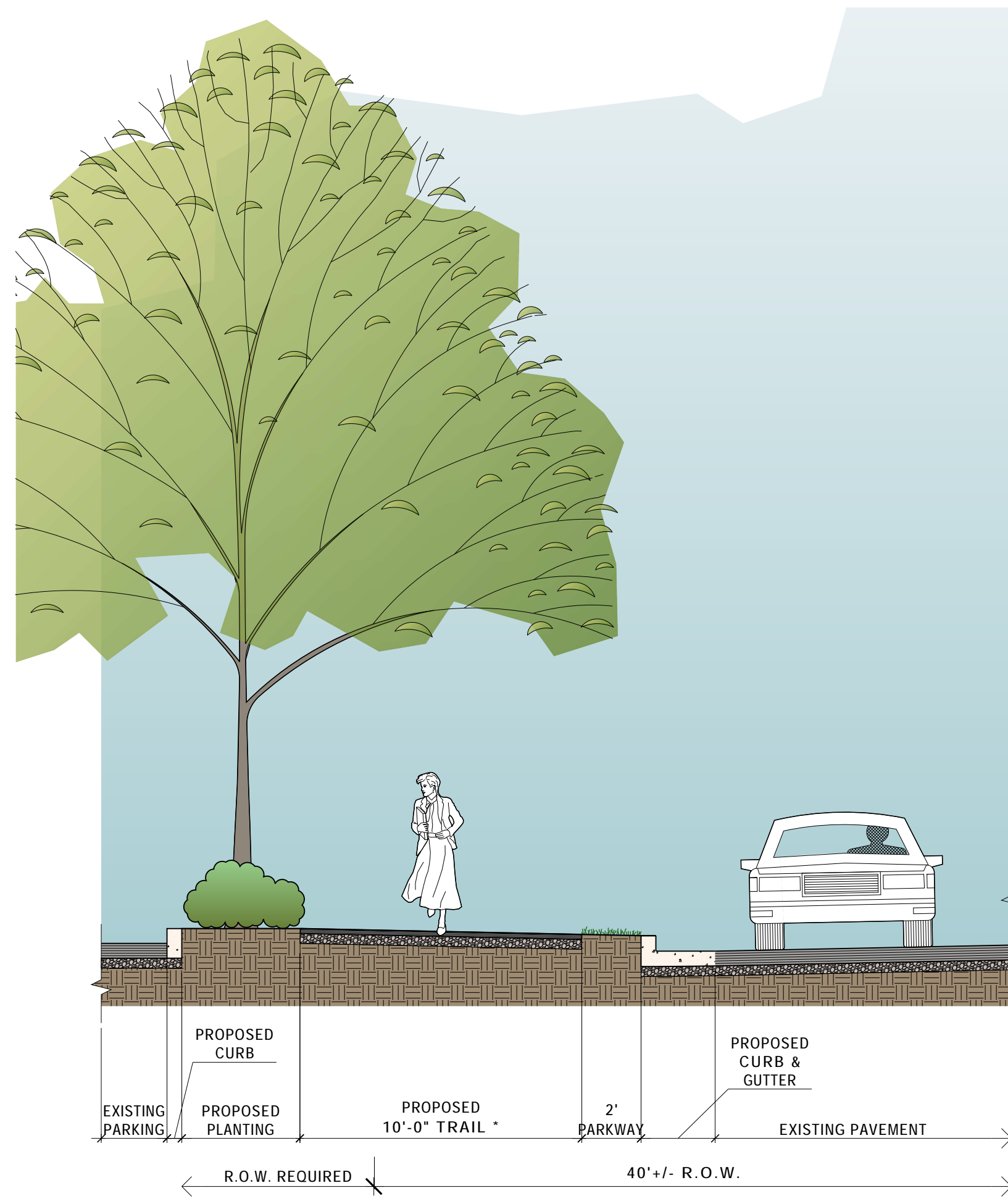
4 TRAIL SECTION @ PARKING LOT SCALE: 1/4"=1'-0"
